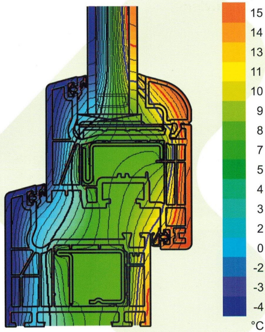
Andamento isotermico Schüco Corona CT 70 AS Classic
